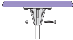
Stools are secured to their columns by an inset washer and a hex bolt with an aircraft lock nut.
